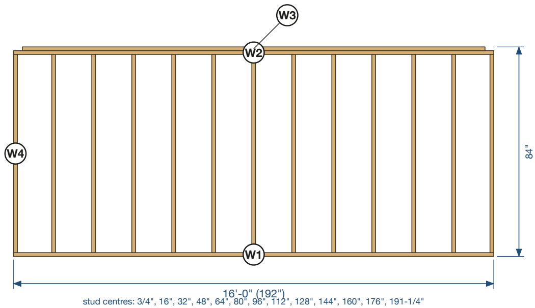
SIDE WALL FRAMING (seen from outside)
