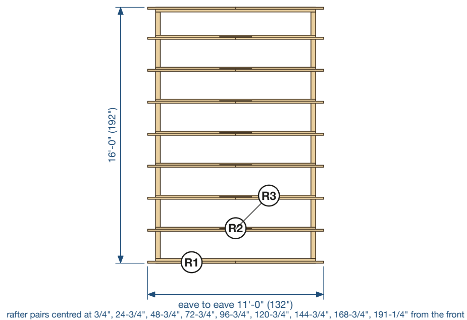
ROOF FRAMING PLAN (from above, roof deck removed)
